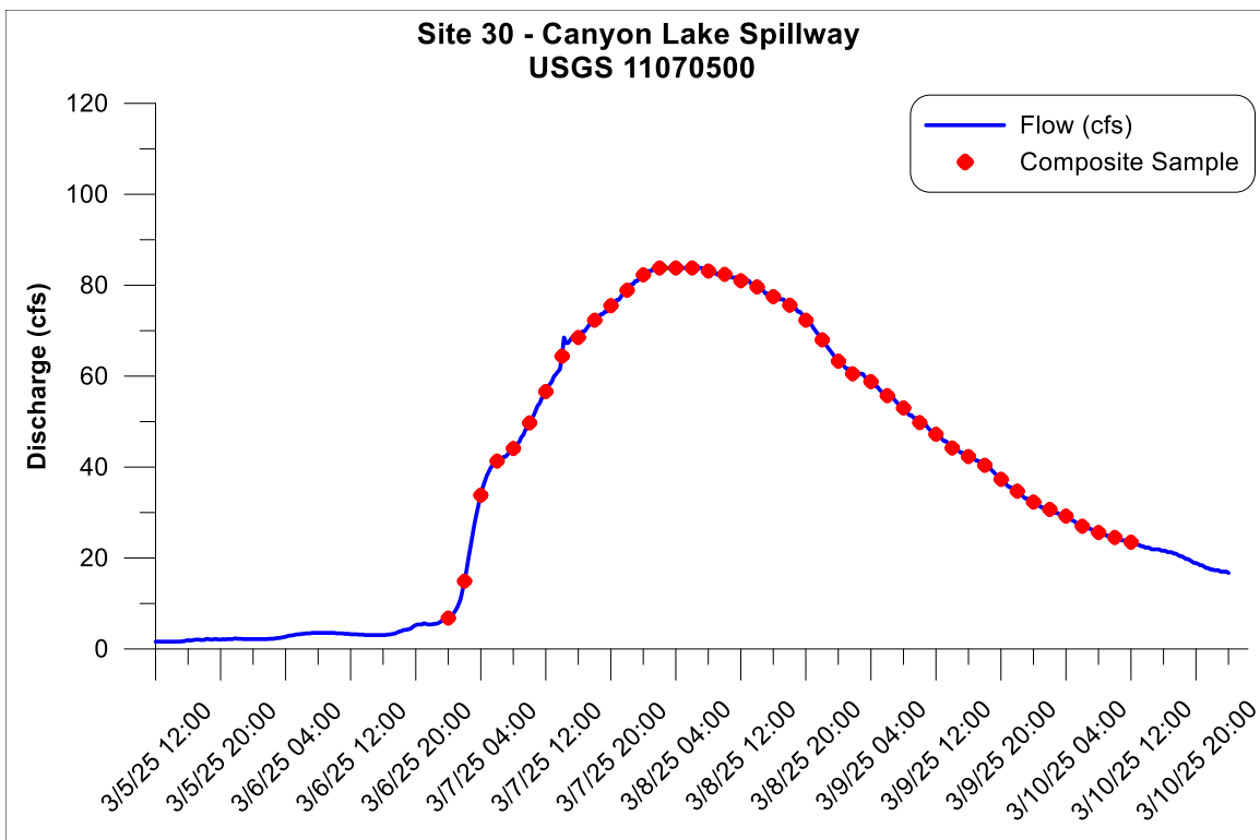
Figure 2-21. Hydrograph of First Storm Event at Canyon Lake Spillway ( March 7-10, 2025)
