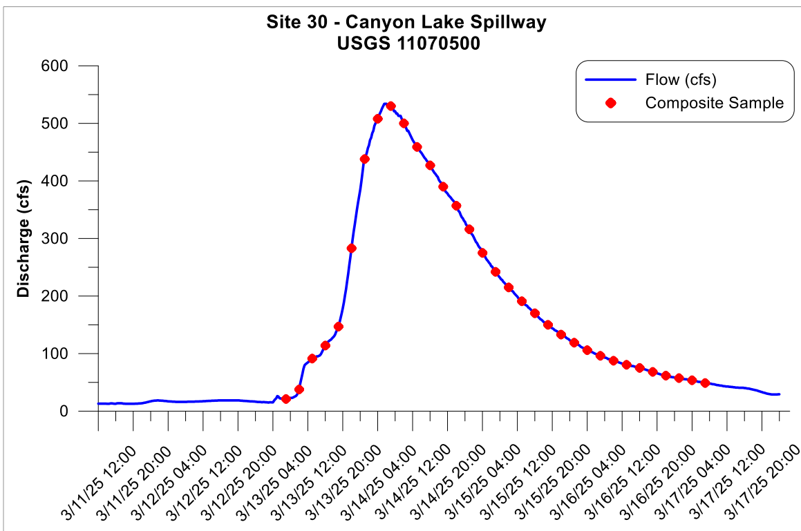
Figure 2-22. Hydrograph of Second Storm Event at Canyon Lake Spillway (March 13-17, 2025)
