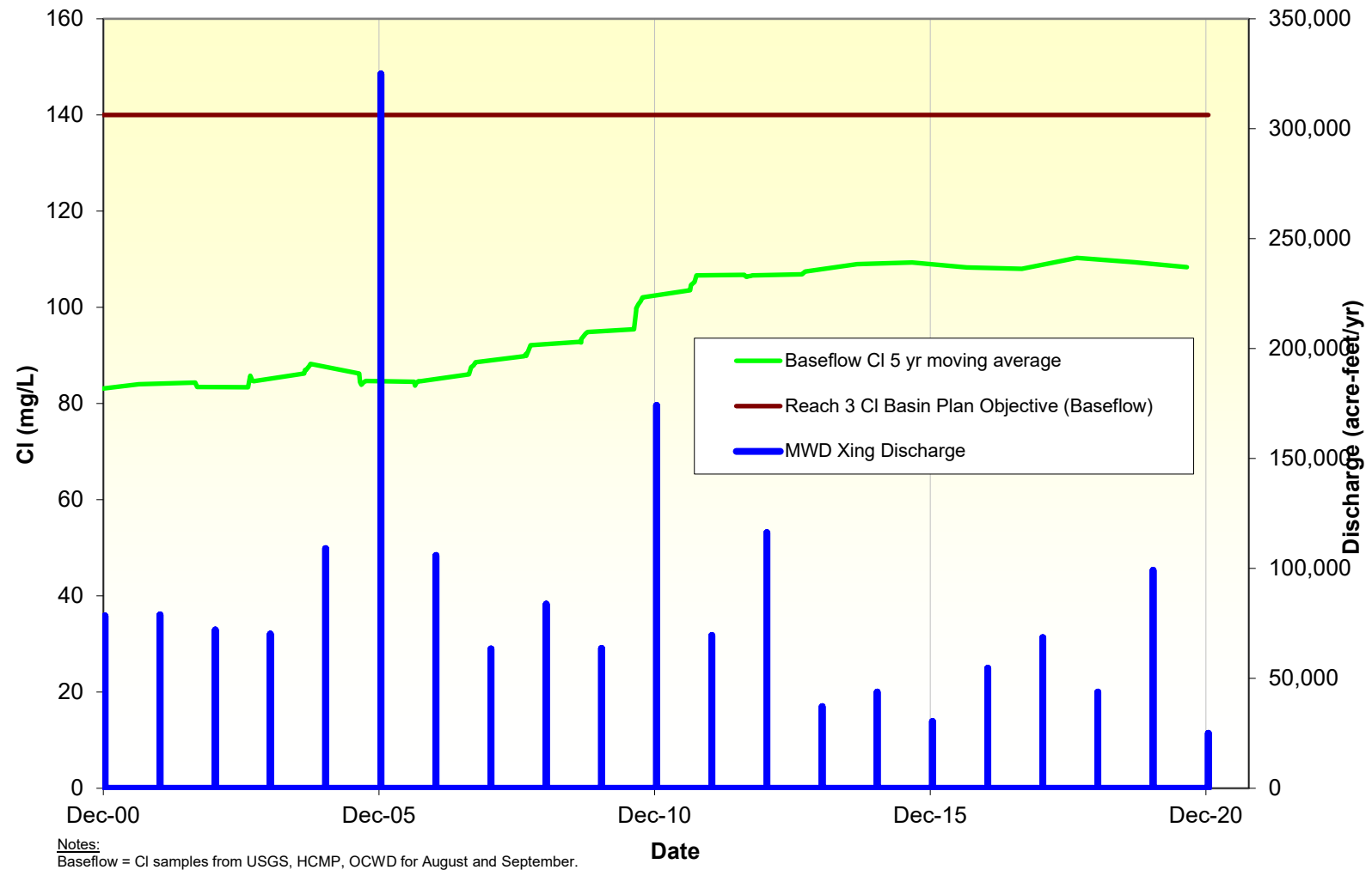
Figure A-11 Chloride (Cl) MWD Crossing
