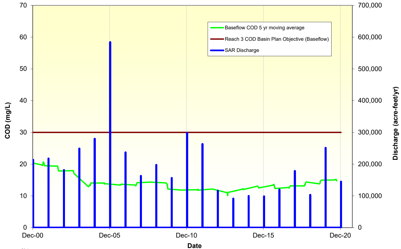
Figure A-4 Chemical Oxygen Demand (COD) Below Prado Dam
