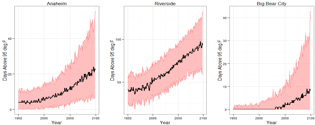
Figure 28: Projected annual number of days above 95°F. Solid black line is the median and the red shading denotes the 5 th and 95 th percentile bounds
