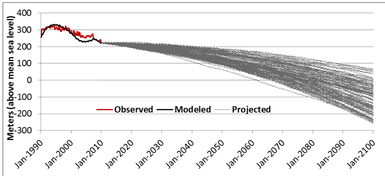
Figure 17: Projected groundwater elevations for Elsinore for a no action scenario
