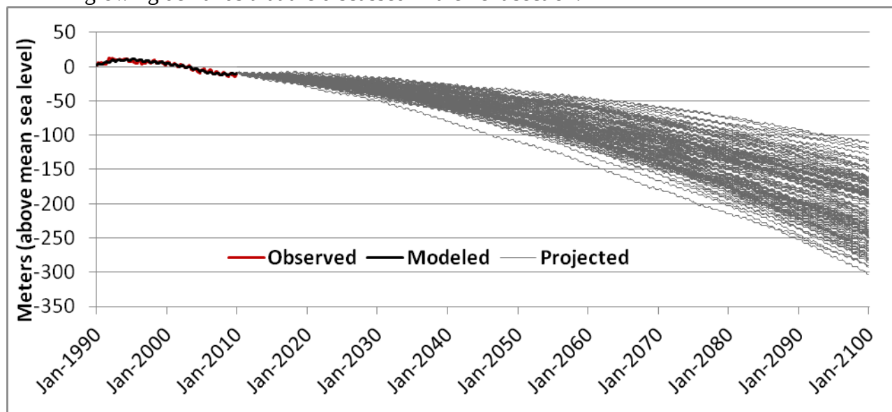
Figure 15: Projected groundwater elevations for Upper Santa Ana Valley for a no action scenario
