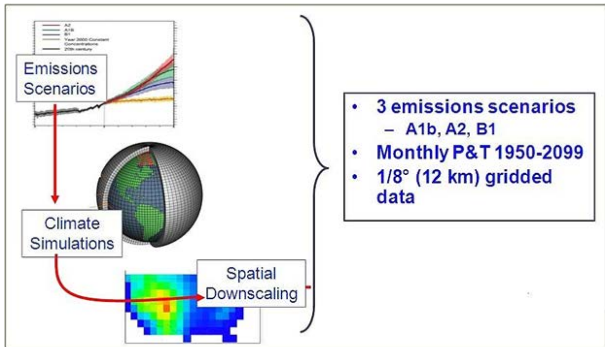
Figure 2: Downscaled GCM key elements
