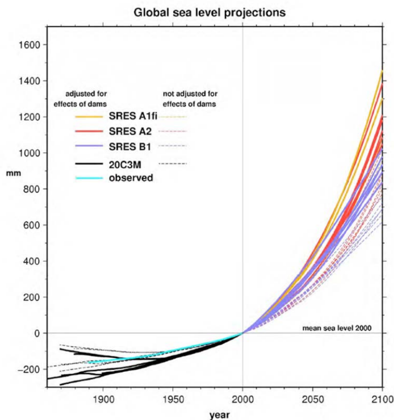
Figure 33: Projections of global mean sea level rise
