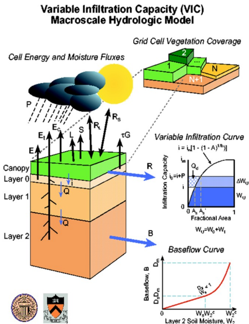
Figure 3: VIC macroscale hydrologic model
