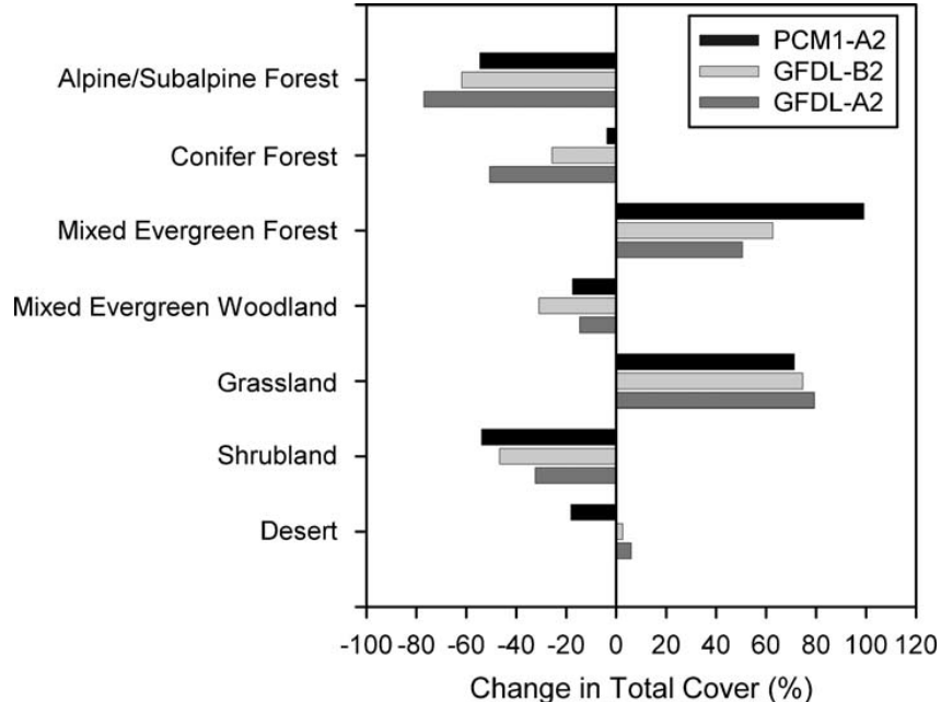
Figure 25: Fig. 4 from Lenihan et al., (2008). Percent change in total land cover for vegetation classes by 2100 for three climate change scenarios predicted using the MC1 Dynamic Vegetation Model
